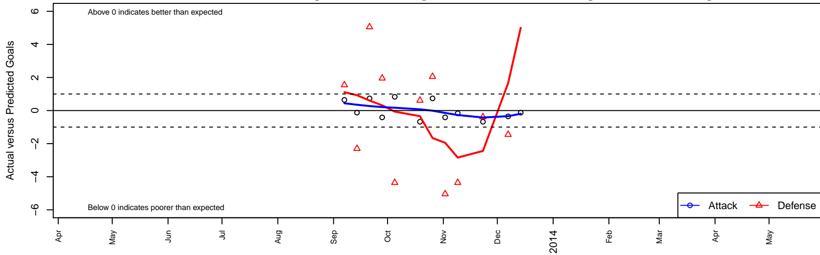
Marysville Force B01 Dots are actual minus expected GF (blue circles) and GA (red triangles). Blue line is smoothed change in attack strength. Red is smoothed change in defense strength.
